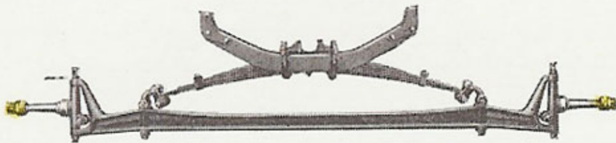
Front axles on all Model T Cars are each drop-forged from one single ingot of Vanadium steel specially heat-treated in our own plant
